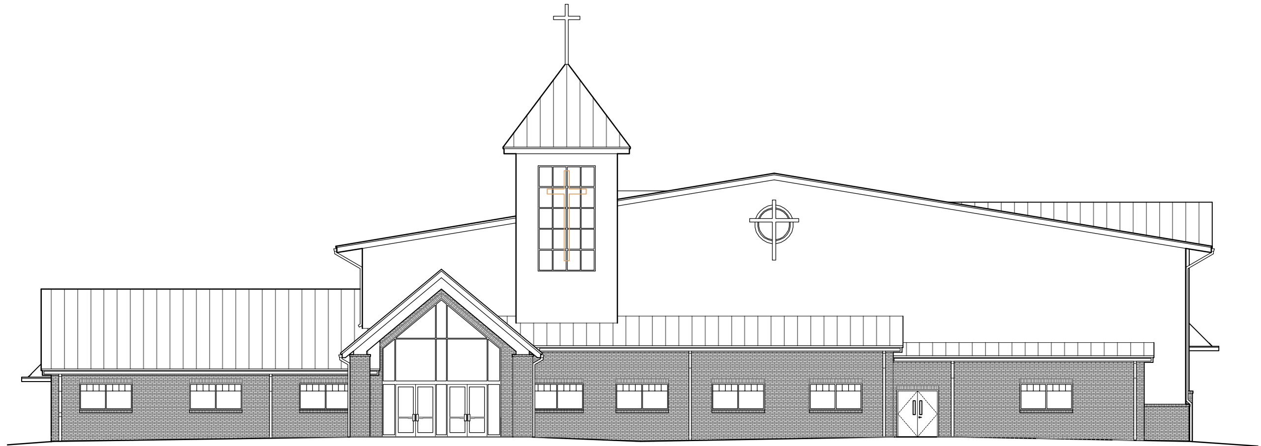
NORTH ELEVATION
